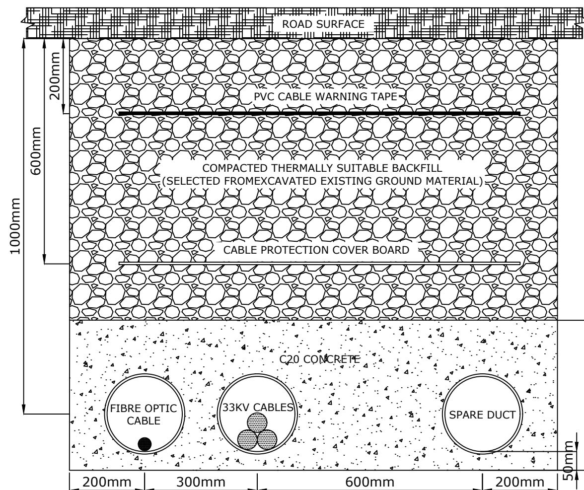
TYPICAL CABLE TRENCH DETAIL AT ROAD CROSSING (1:10)
